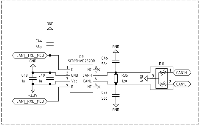
CAN 1
